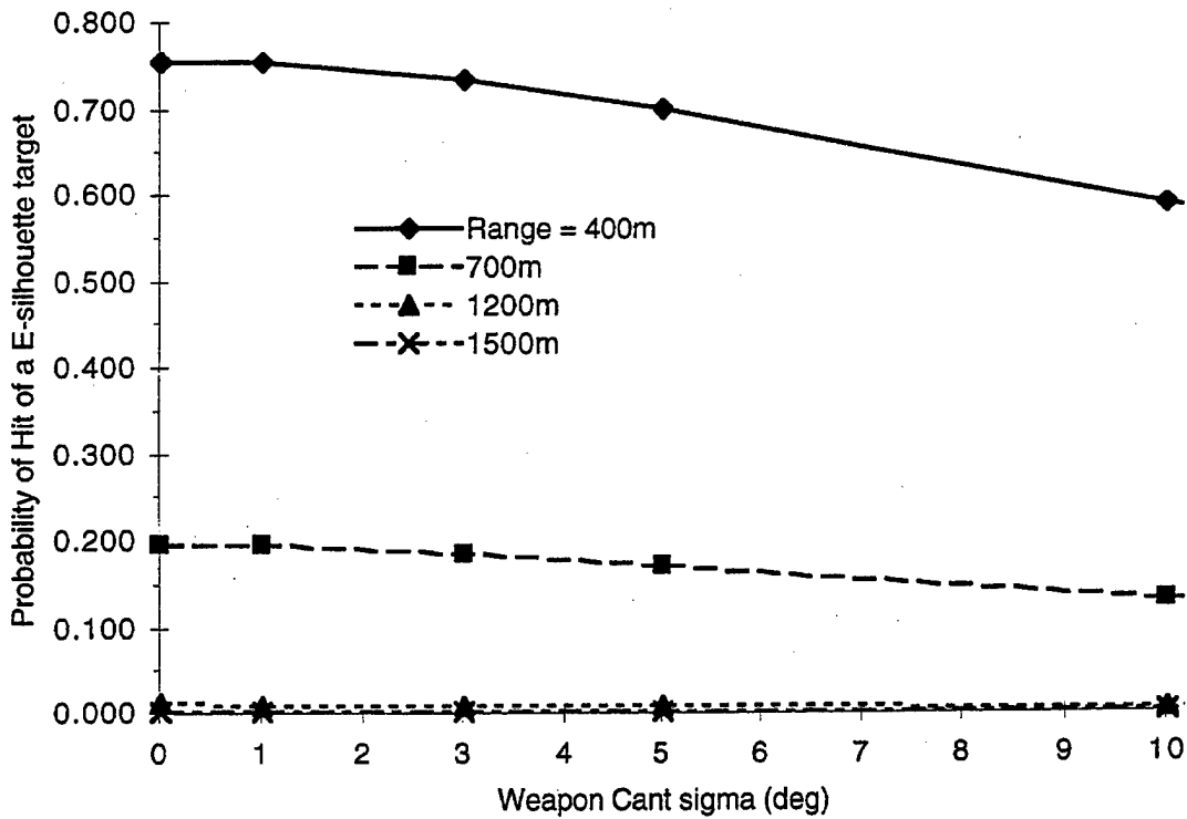
Figure D-2. Error Budget Sensitivity, Weapon Cant.
